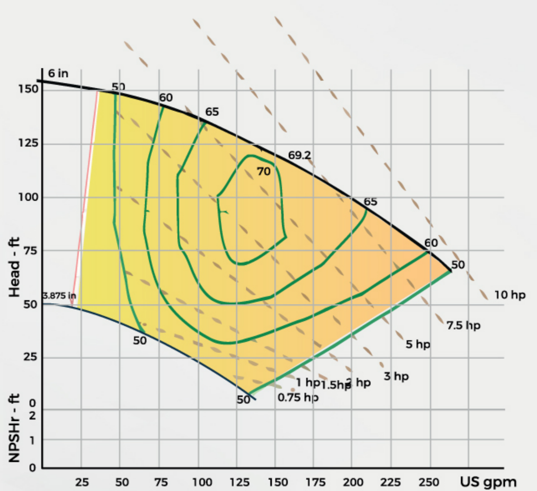
PUMP SIZE 1.5X2-6
