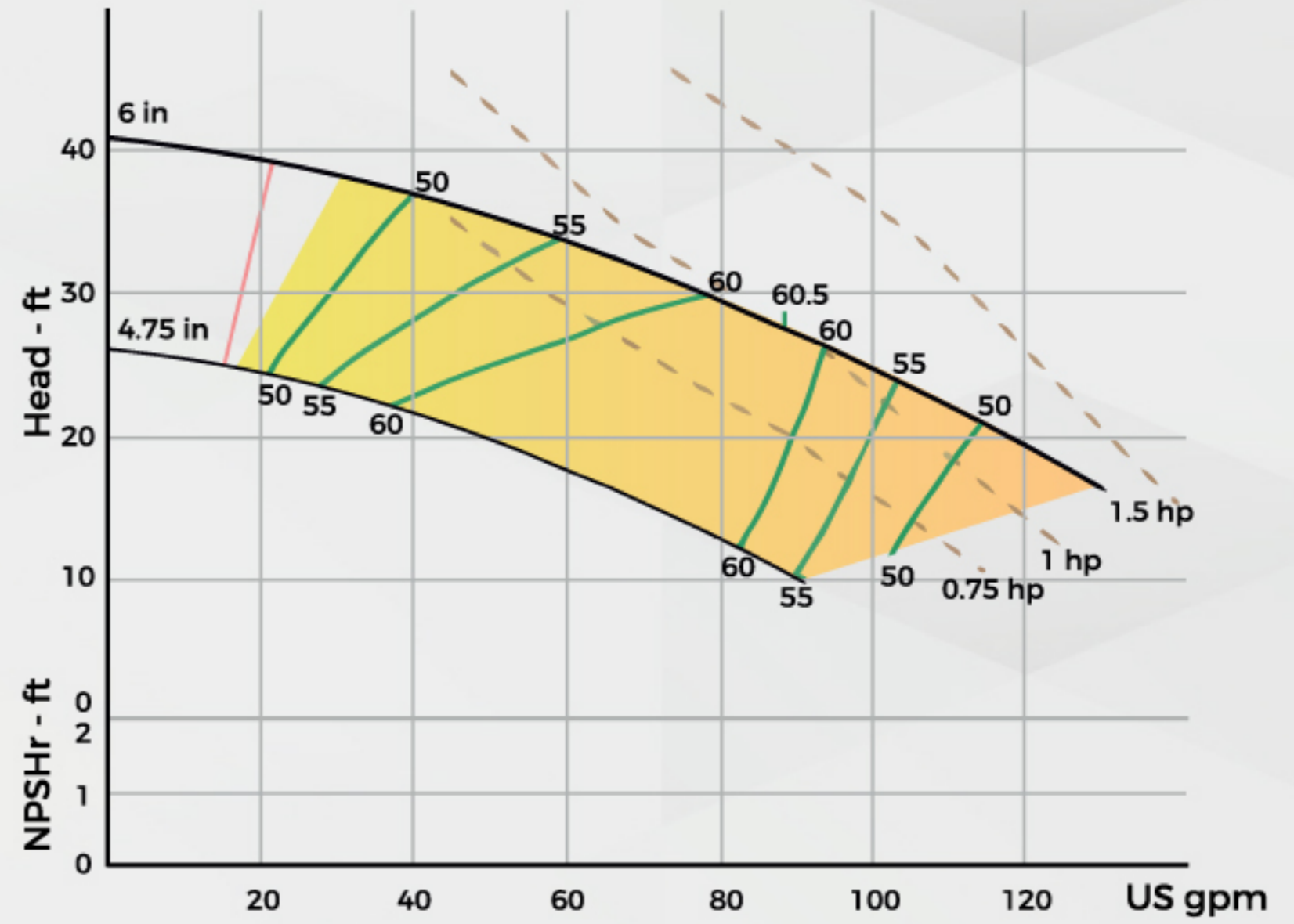
PUMP SIZE 1.5X2-6
