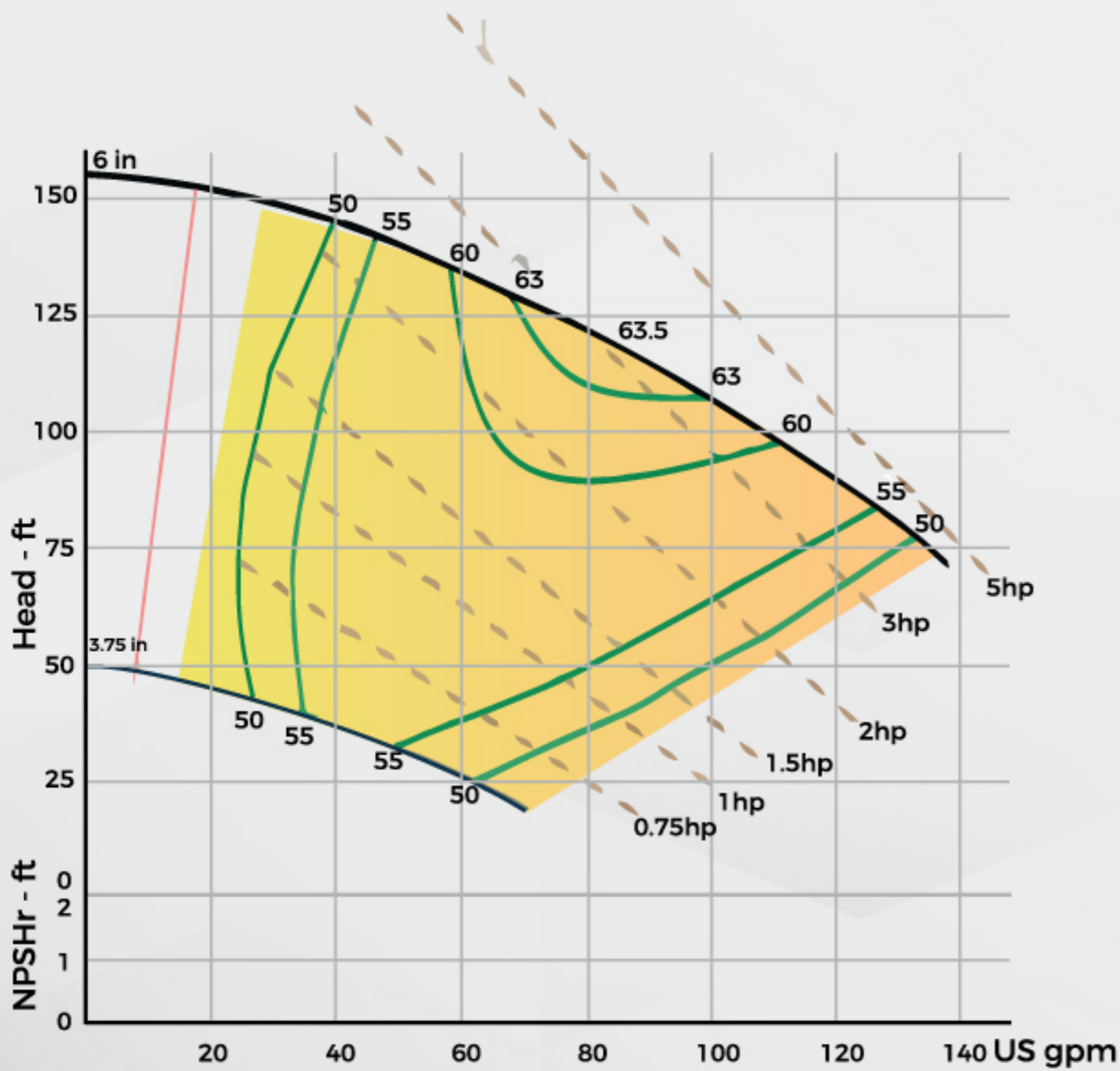
PUMP SIZE 1X1.5-6
