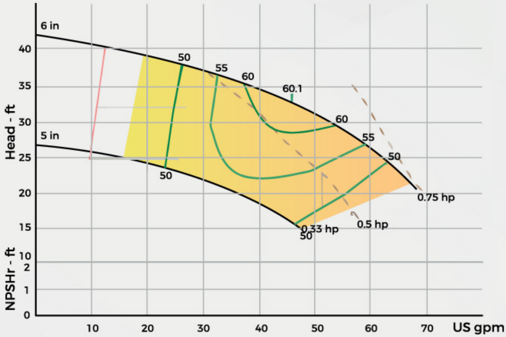
PUMP SIZE 1X1.5-6
