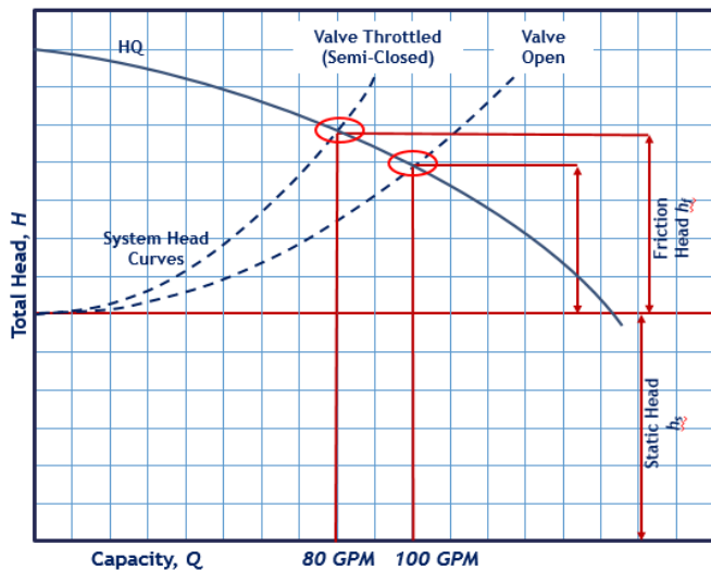
Figure 3: Friction Head Curve
