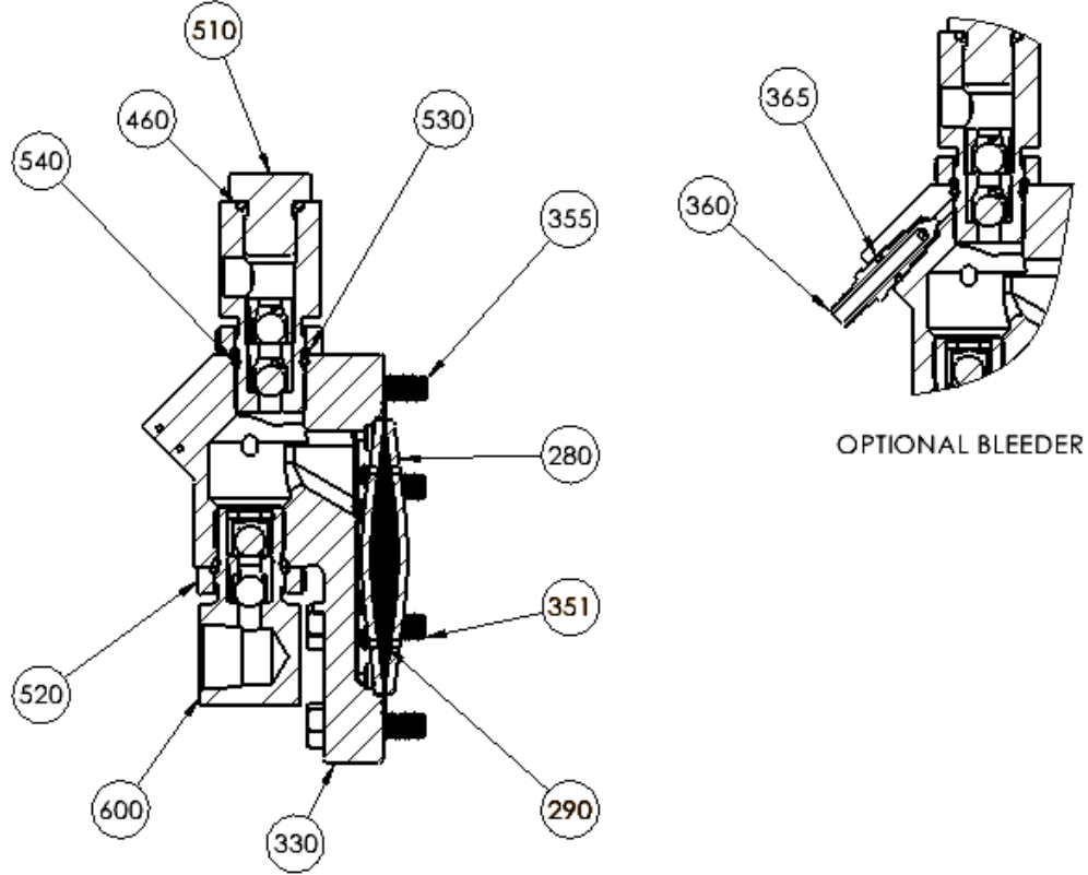
mRoy A: E, F PLUNGER LIQUID ENDS (DWG 9992004017)
