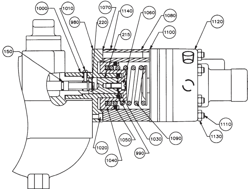
PNEUMATIC CAPACITY CONTROL
