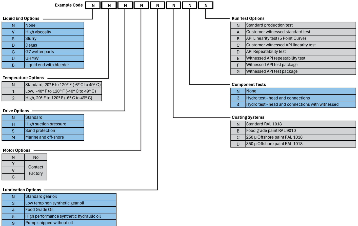
FIGURE 4. GLOBAL MRA/MRB MODEL CODE EXTRA
