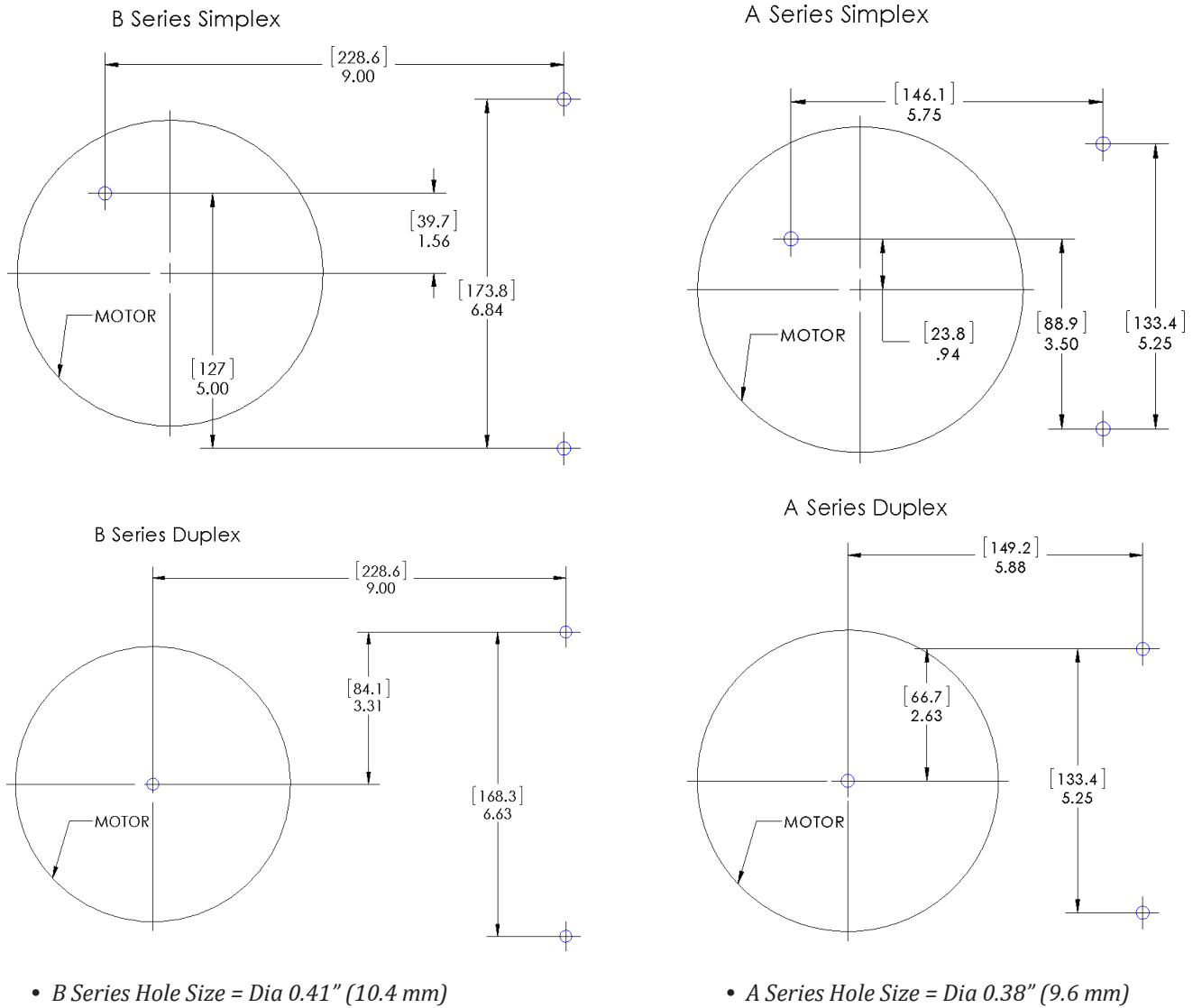
FIGURE 11. MOUNTING BOLT HOLES
