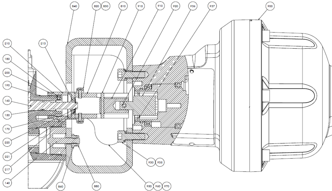
ACTUATOR CAPACITY CONTROL
