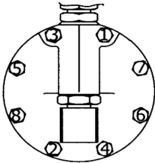
mRoy A- 8 Bolt Pattern
