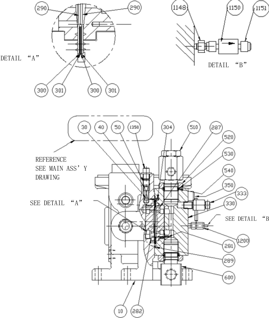
FIGURE 20. MROY A DOUBLE DIAPHRAGM AND LEAK DETECTION
