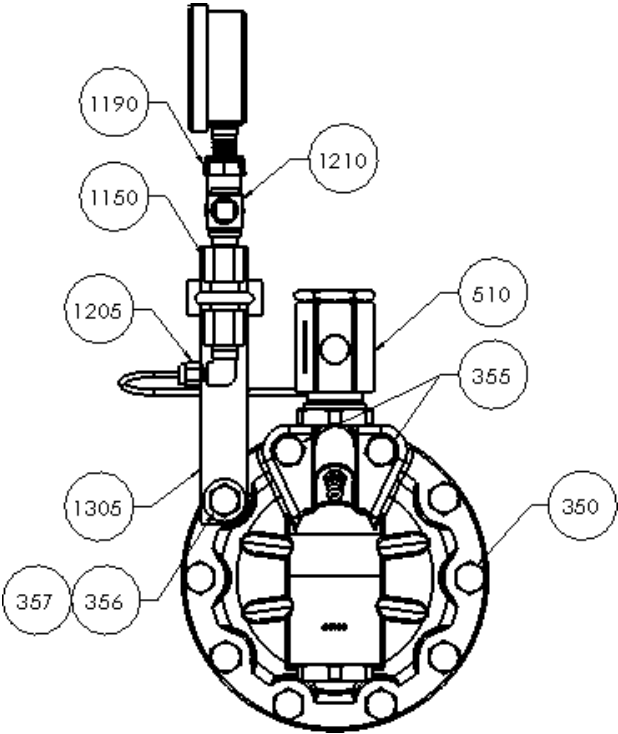
FIGURE 25. MROY B LEAK DETECTION WITH SWITCH AND GAUGE (DWG 99920100005)
