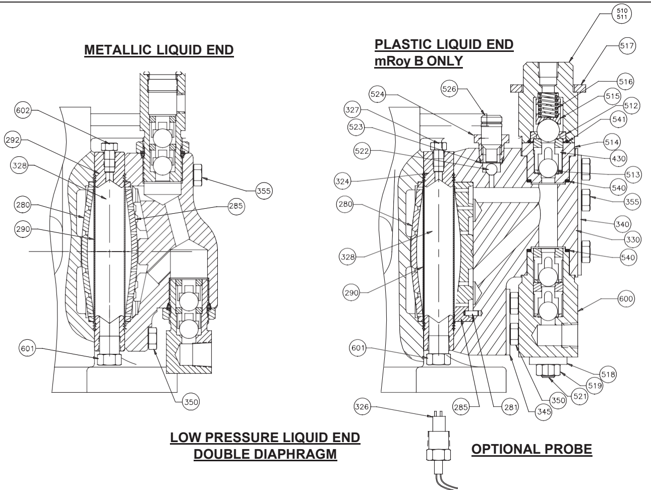
FIGURE 29. MROY B DOUBLE DIAPHRAGM (DWG 99920100025 & 99920100026)
