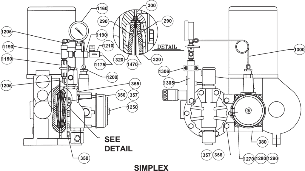
FIGURE 25. MROY B LEAK DETECTION WITH SWITCH AND GAUGE (DWG 99920100005)
