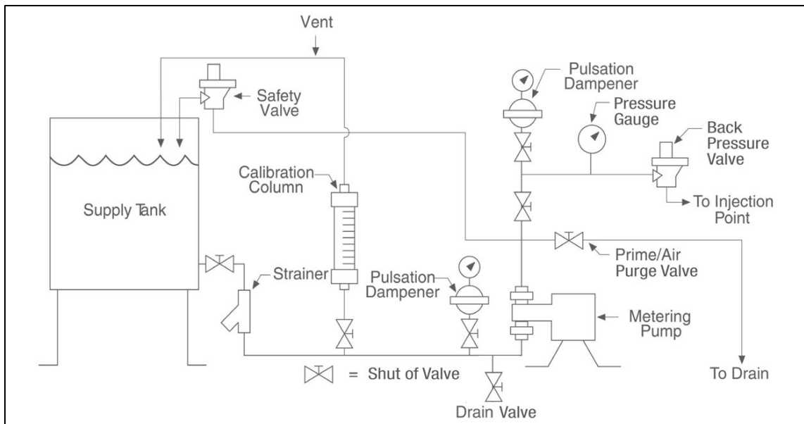
FIGURE 12. TYPICAL PIPING AND INSTRUMENTATION DIAGRAM
