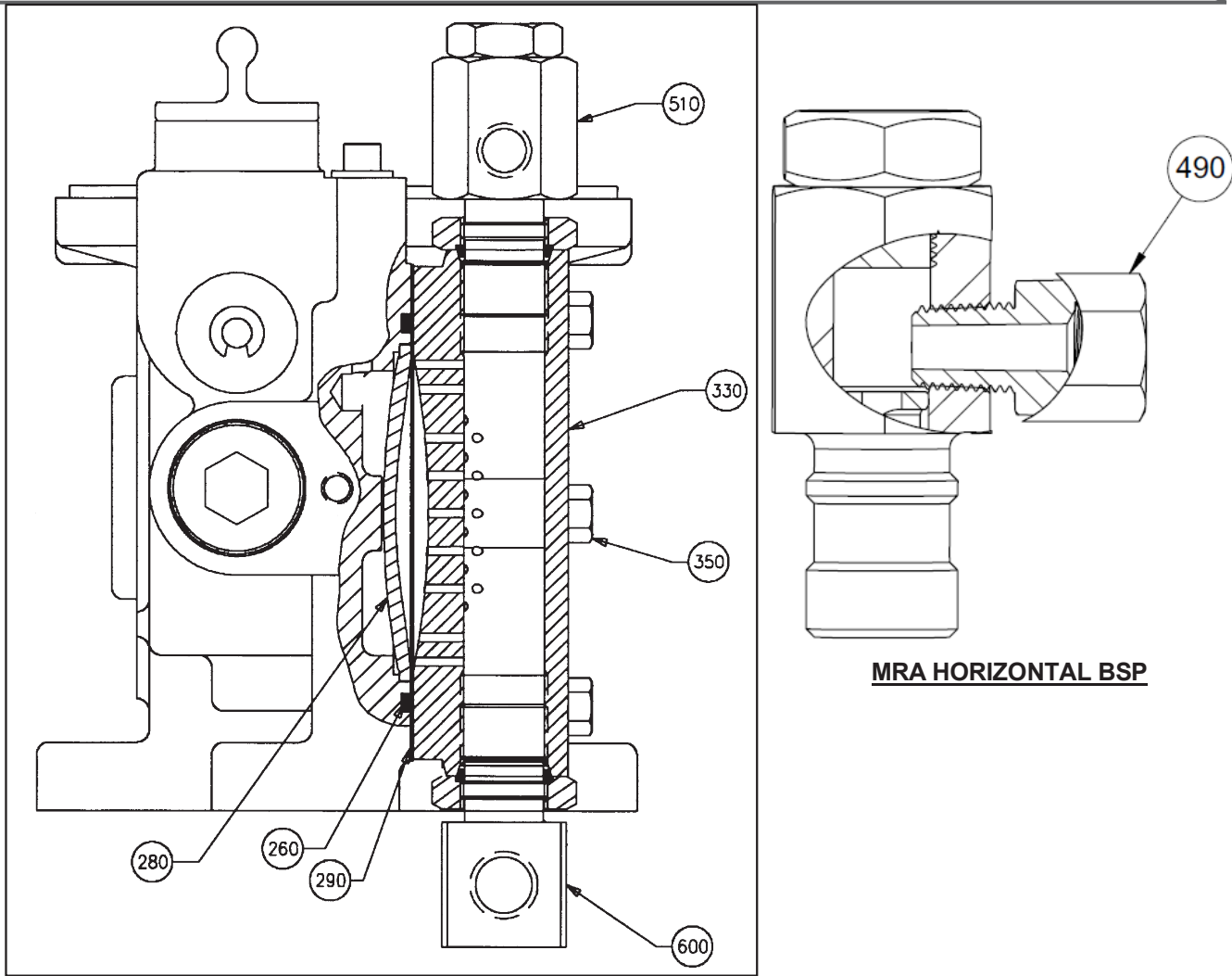
BAR STOCK LIQUID END
