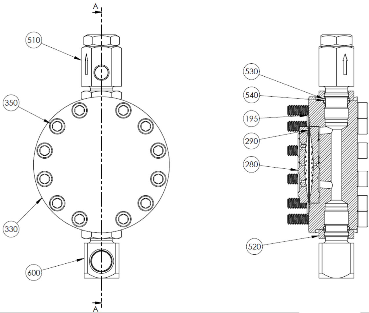
FIGURE 27. MROY B PLUNGER "H" 316SS LIQUID END (DWG 9994027404)
