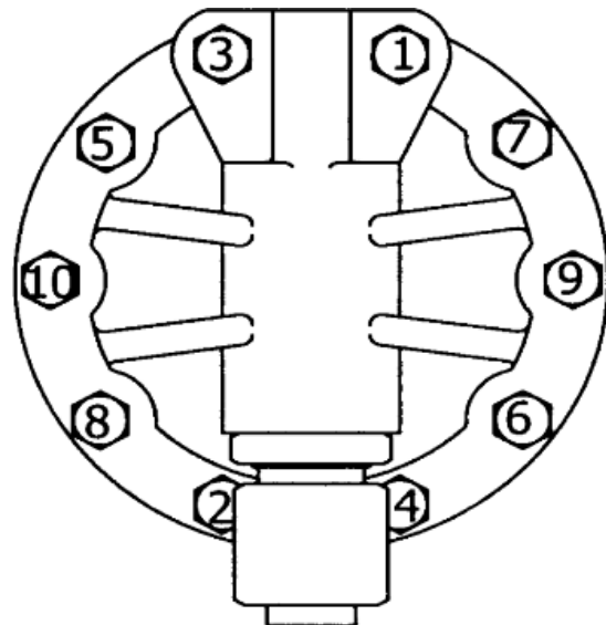
mRoy B- 10 Bolt Pattern
