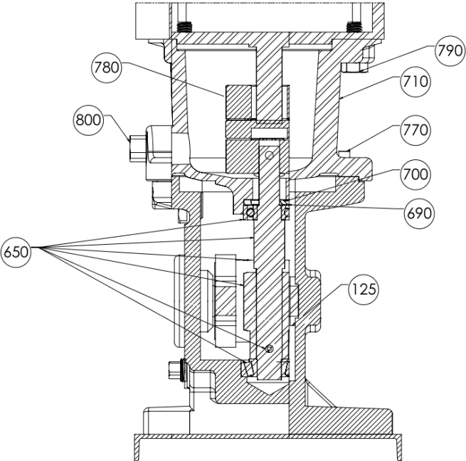
API FLANGE MOTOR MOUNT
