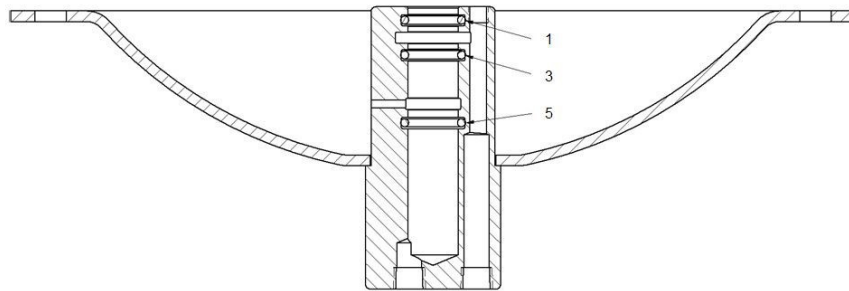
Figure 1: AODDampener Automatic Valve O-Rings
