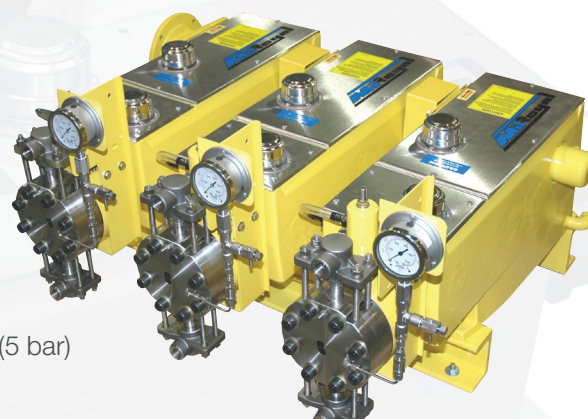
MILROYAL B Triplex with leak detection
