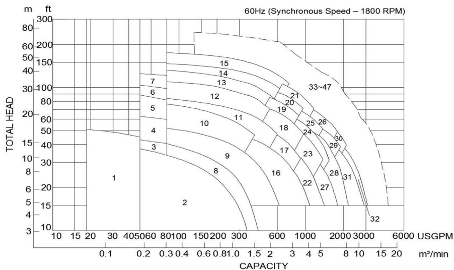
Three Phase 60Hz
