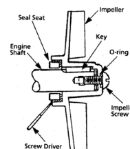
Figure 1 - Mechanical Seal Replacement
